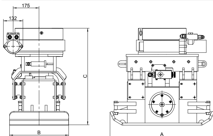
MAV 08 with RD 12 Worm Gear
